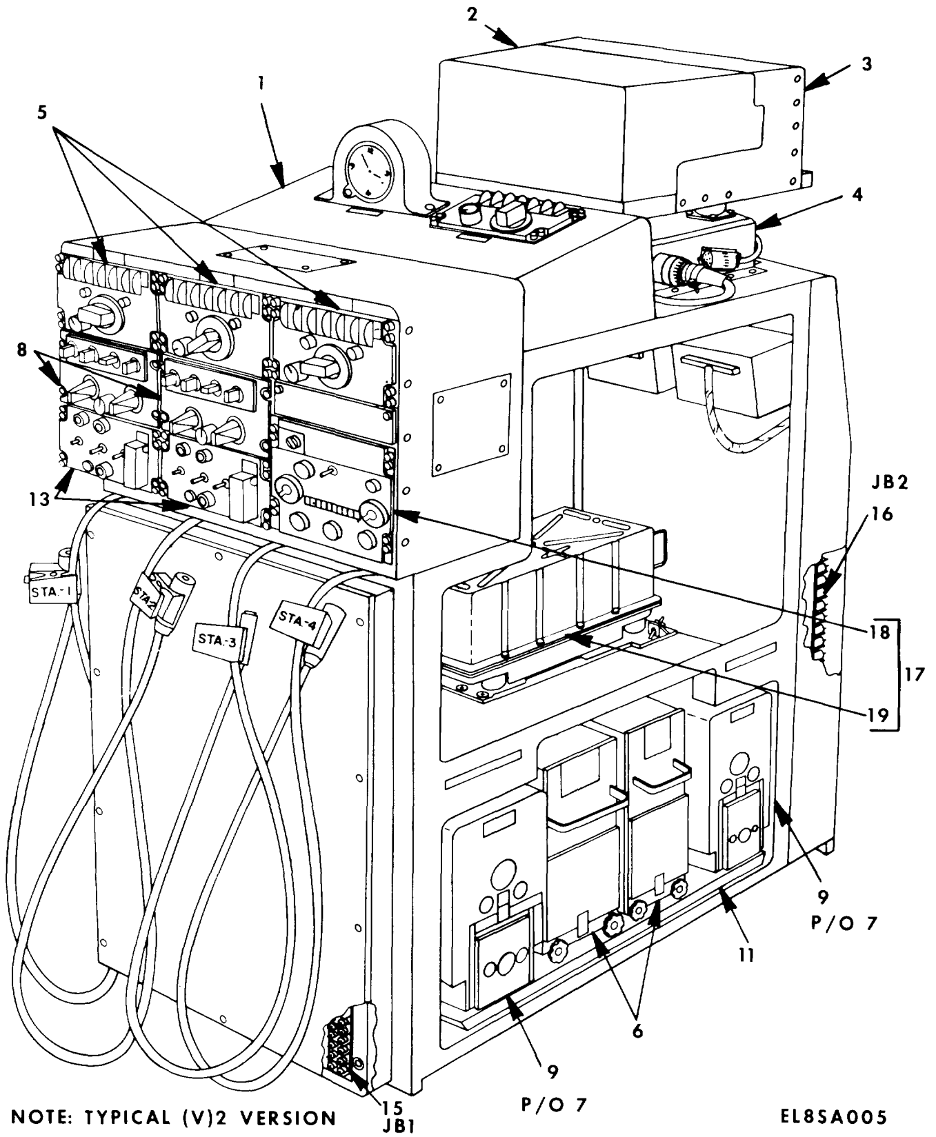
Figure 1. Communications Central AN/ASC-15(V)1 and 2 (Sheet 5 of 9).
