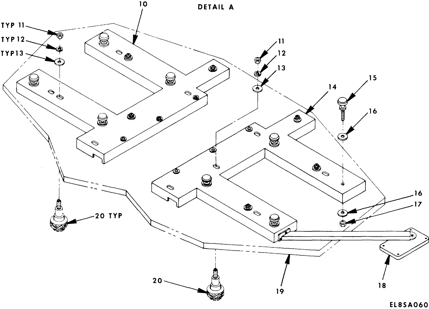
Figure 17. AN/ASC-15A V1 and V2 Installation Kit UH-1D/H (Sheet 2 of 4).
