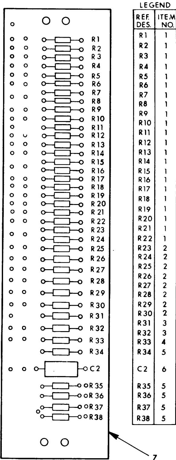
Figure 26. Audio Pad Assembly.
