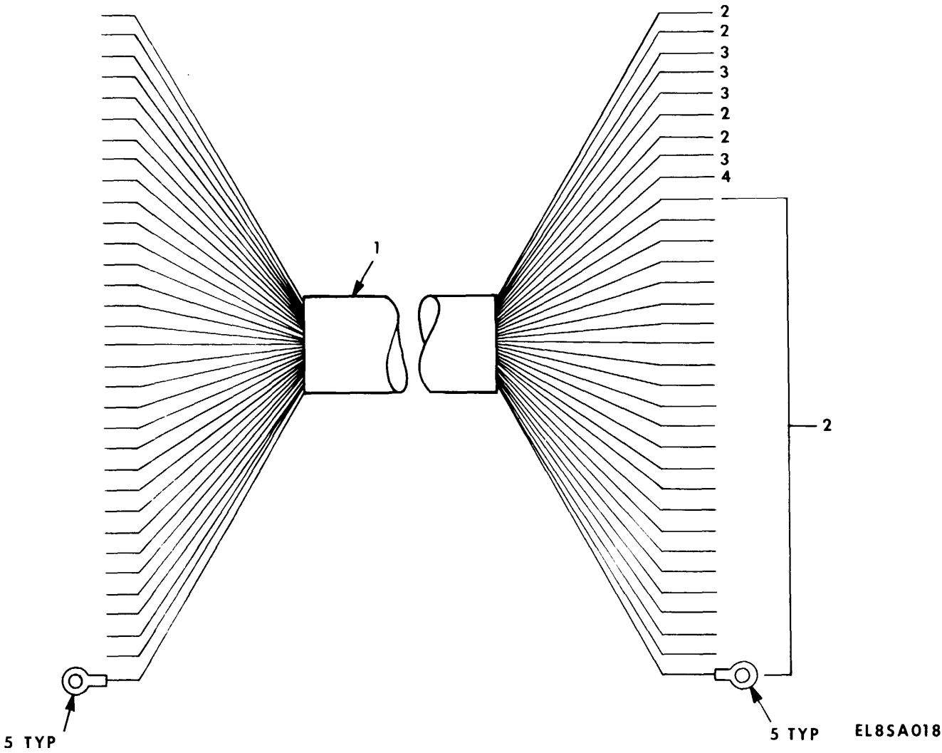
Figure 7. Cable Assembly (Junction Box) (Sheet 1 of 2).
