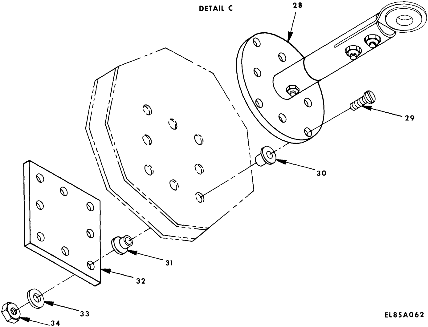
Figure 17. AN/ASC-15A V1 and V2 Installation Kit UH-1D/H (Sheet 4 of 4).
