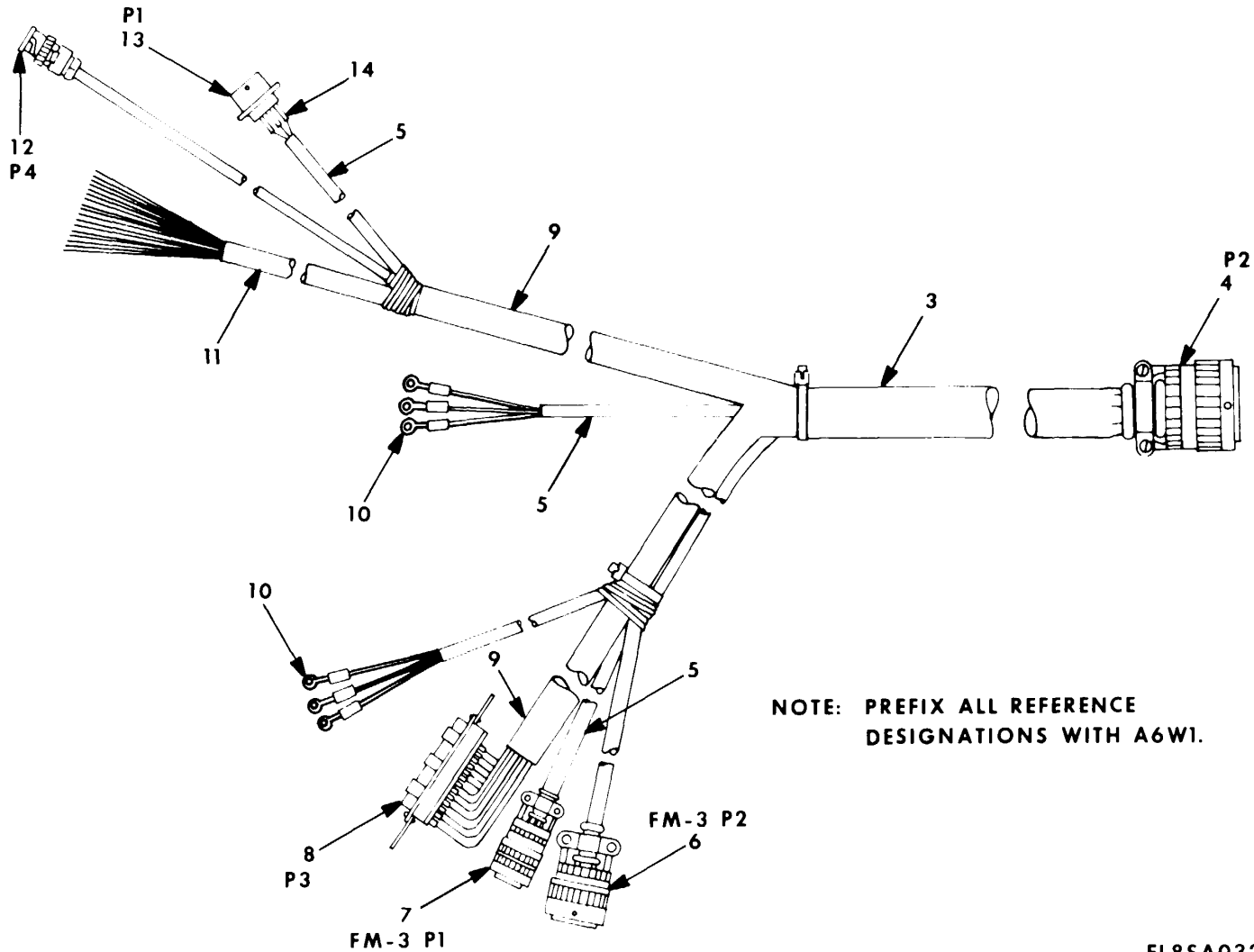
Figure 9. Control Cable Assembly (FM-3, ARC-131 and KY-28) (Sheet 2 of 6).
