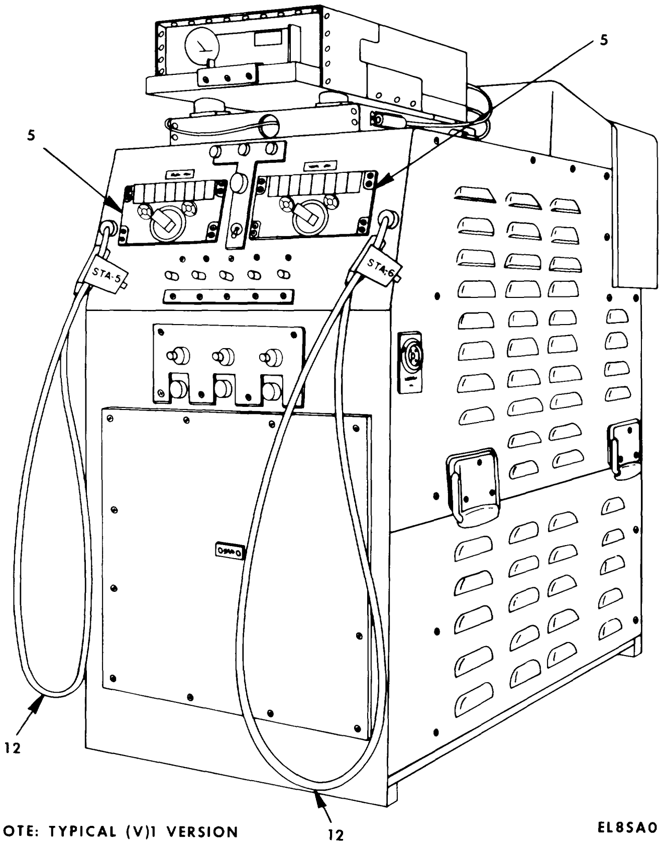
Figure 1. Communications Central AN/ASC-15(V)1 and 2 (Sheet 3 of 9).
