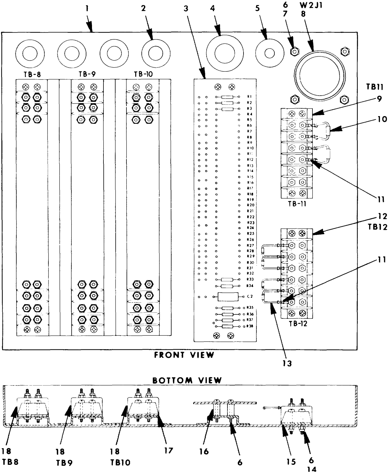
Figure 25. Radio Junction Box Assembly.
