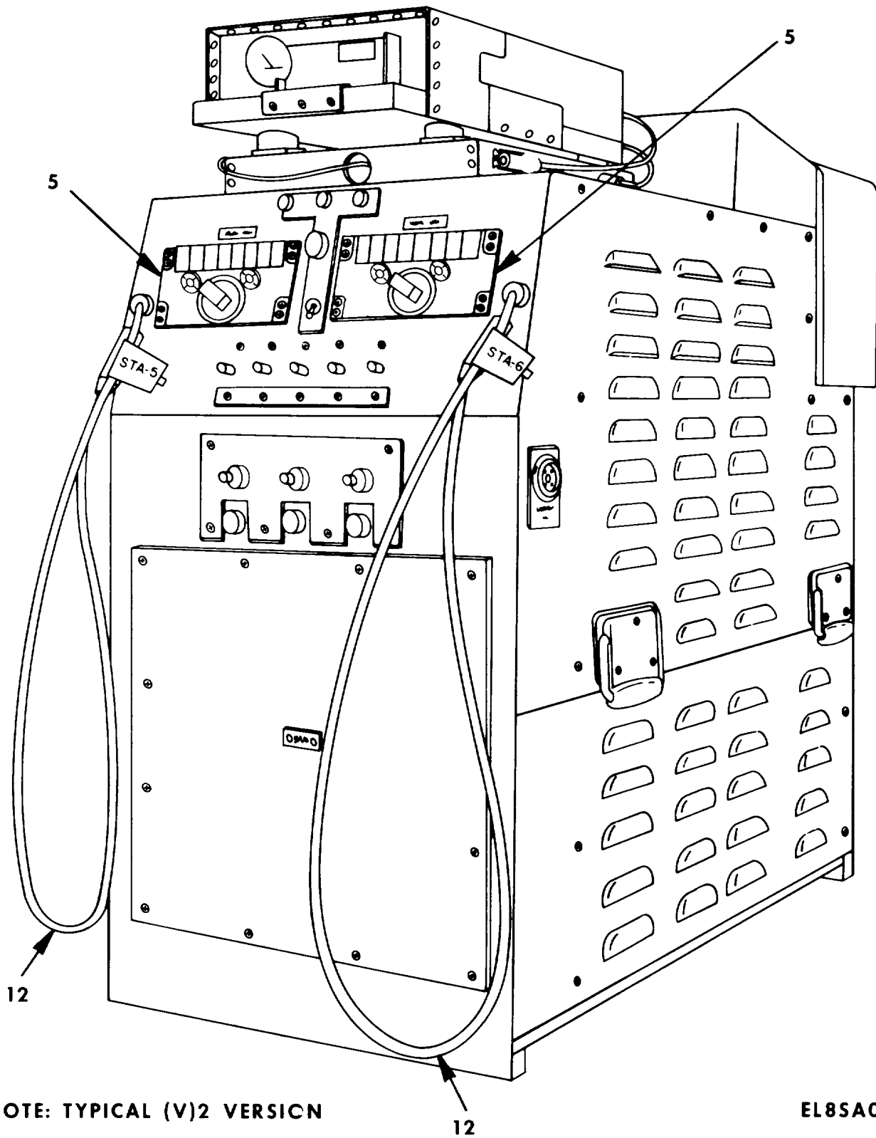
Figure 1. Communications Central AN/ASC-15(V)1 and 2 (Sheet 6 of 9).
