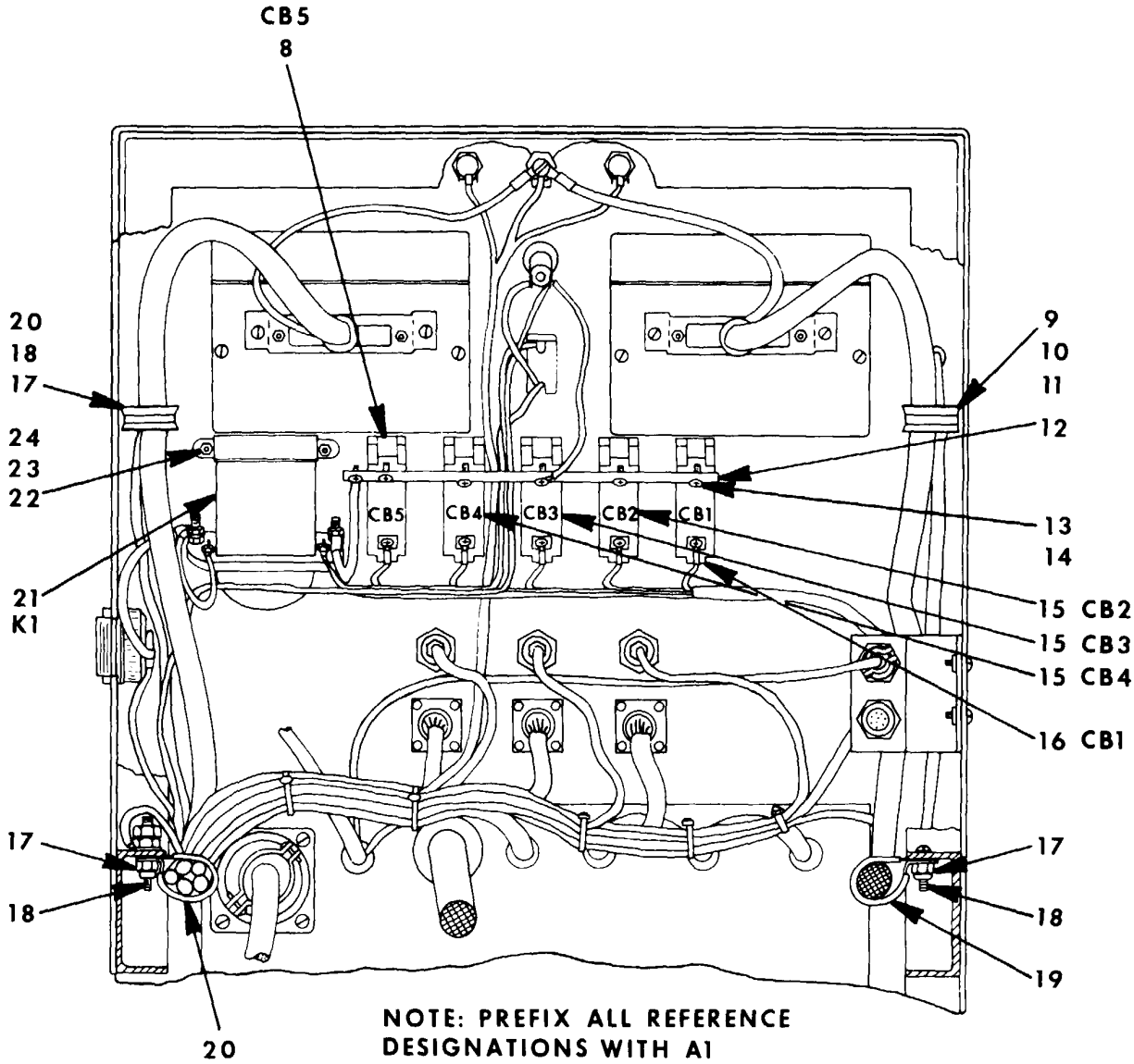
Figure 16. Frame Assembly (V)1 and 2 (Sheet 2 of 6).
