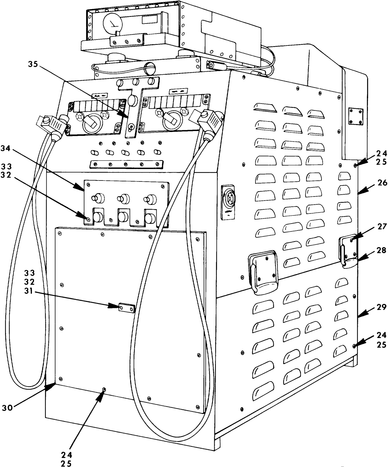
Figure 16. Frame Assembly (V1 and 2 (Sheet 3 of 6).
