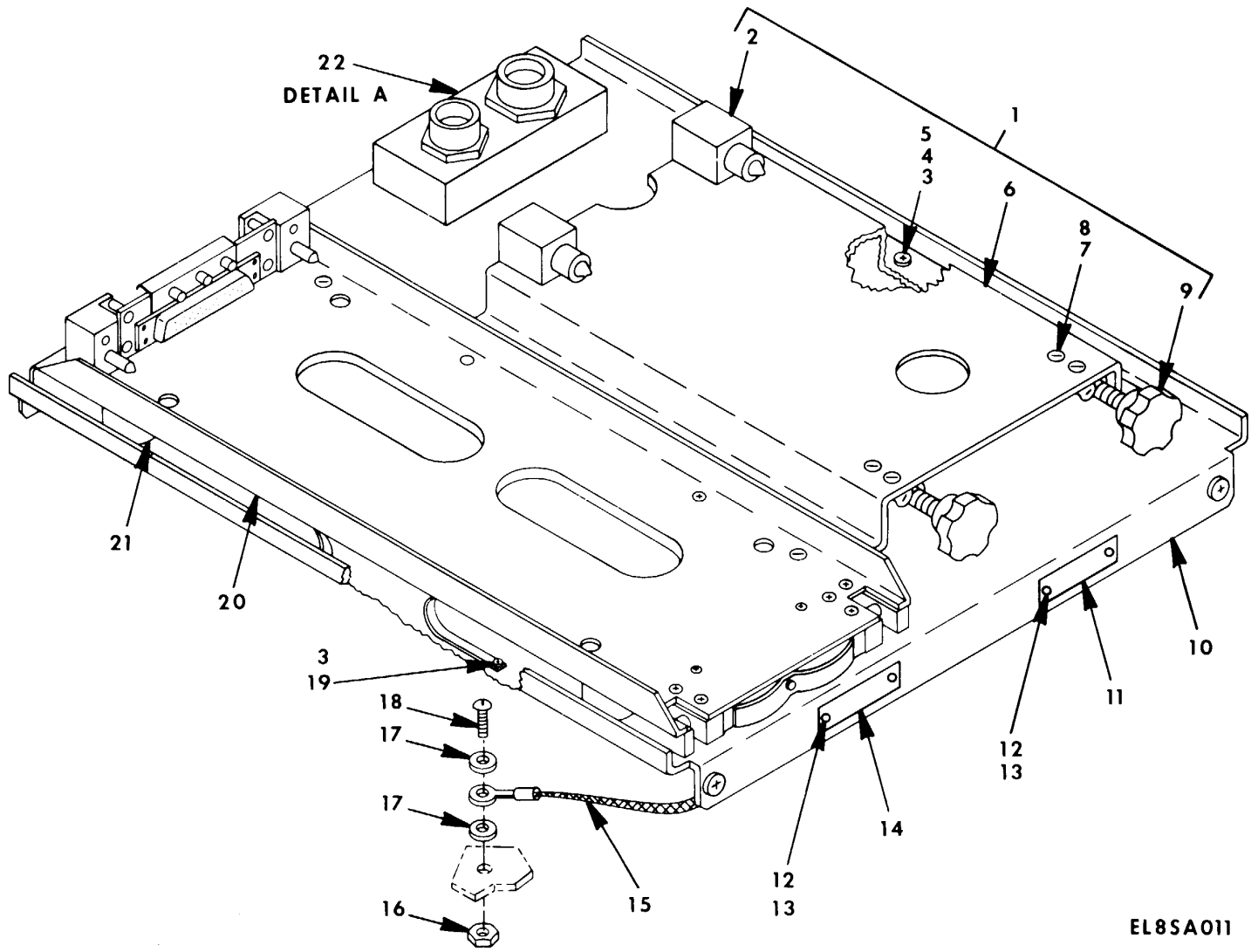
Figure 3. Base Plate Assembly (Upper) (V1 Only) (Sheet 1 of 2).
