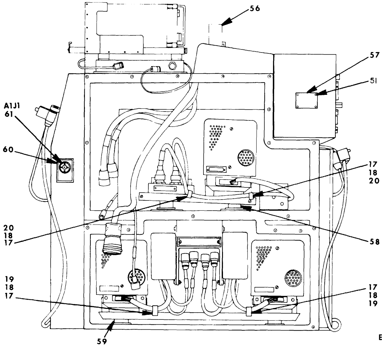
Figure 16. Frame Assembly (V)1 and 2 (Sheet 6 of 6).
