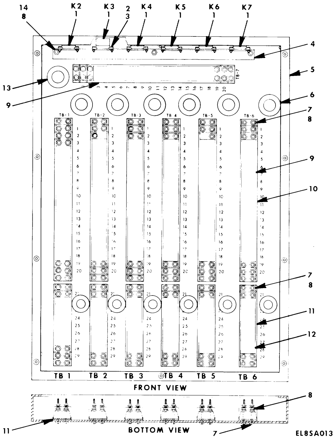
Figure 4. Box Assembly (Interphone Junction)
