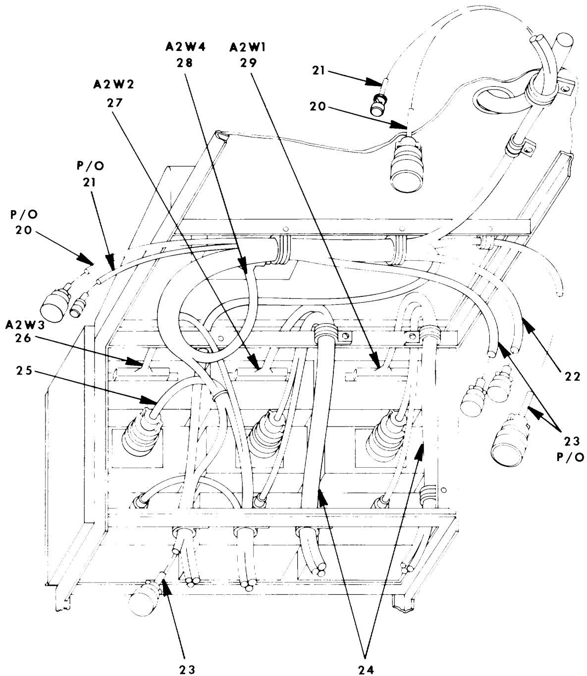
Figure 1. Communications Central AN/ASC-15(V)1 and 2 (Sheet 7 of 9).
