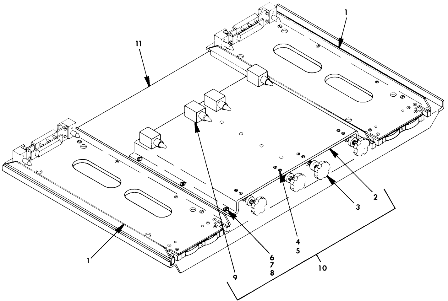
Figure 2. Base Plate Assembly (Lower) and Mounting Plate Assembly (Lower).
