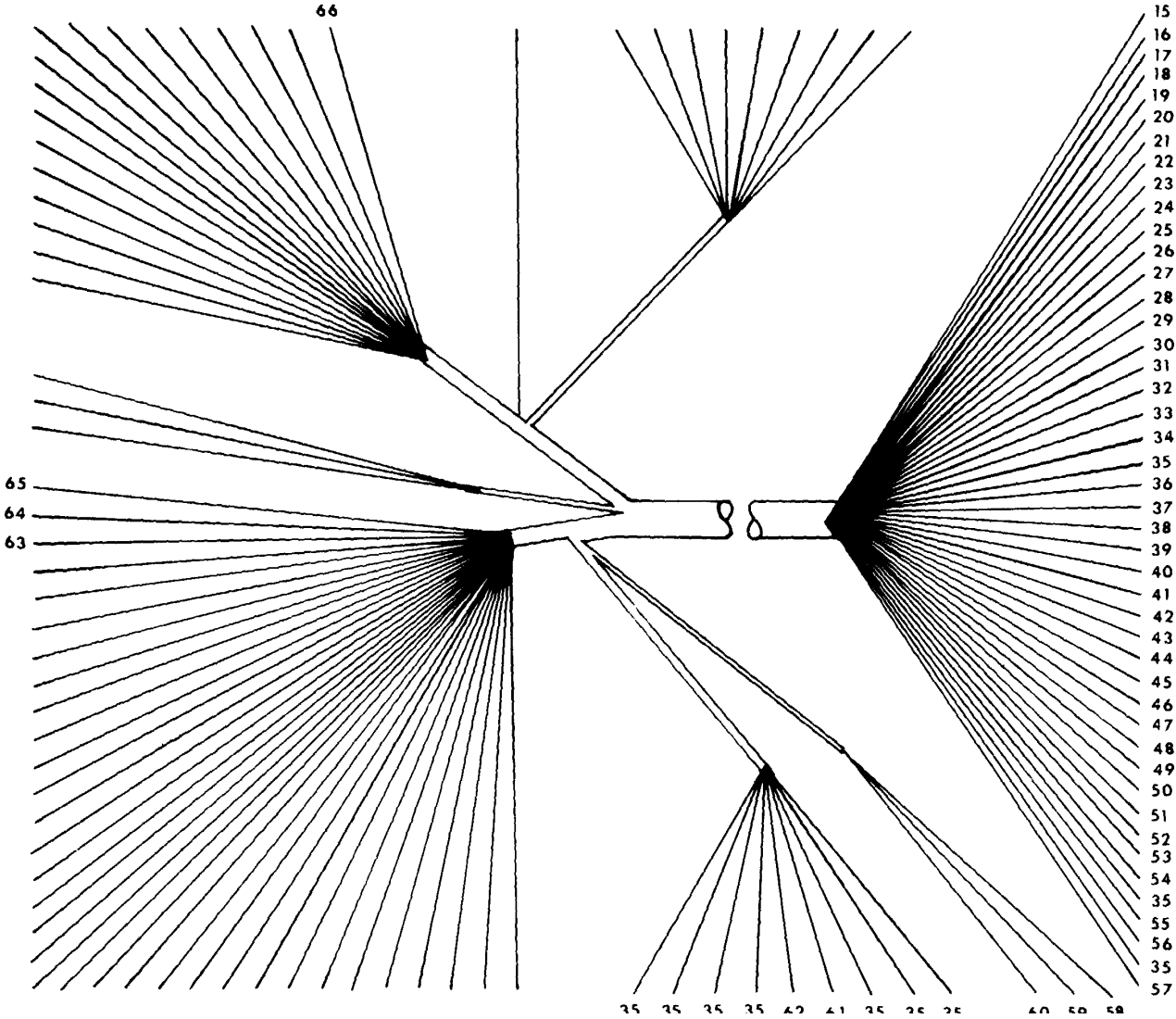
Figure 9. Control Cable Assembly (FM-3, ARC-131 and KY-28) (Sheet 3 of 6).
