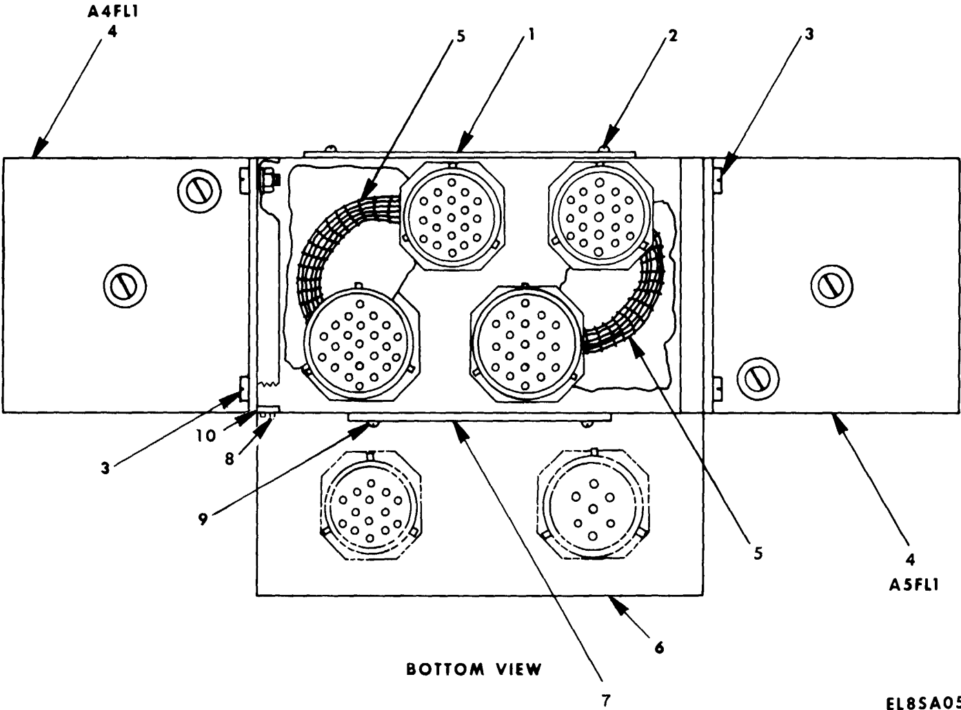
Figure 14. Connector Cover and Bracket Assembly KY-28.
