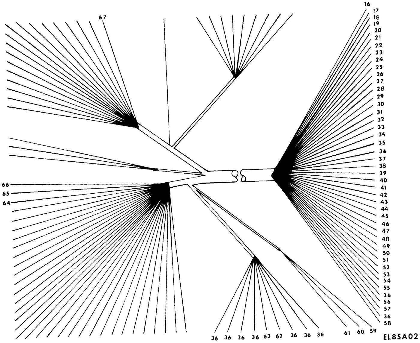
Figure 8. Control Cable Assembly (FM-1, FM-2, ARC-131 and KY-28) (Sheet 3 of 11).
