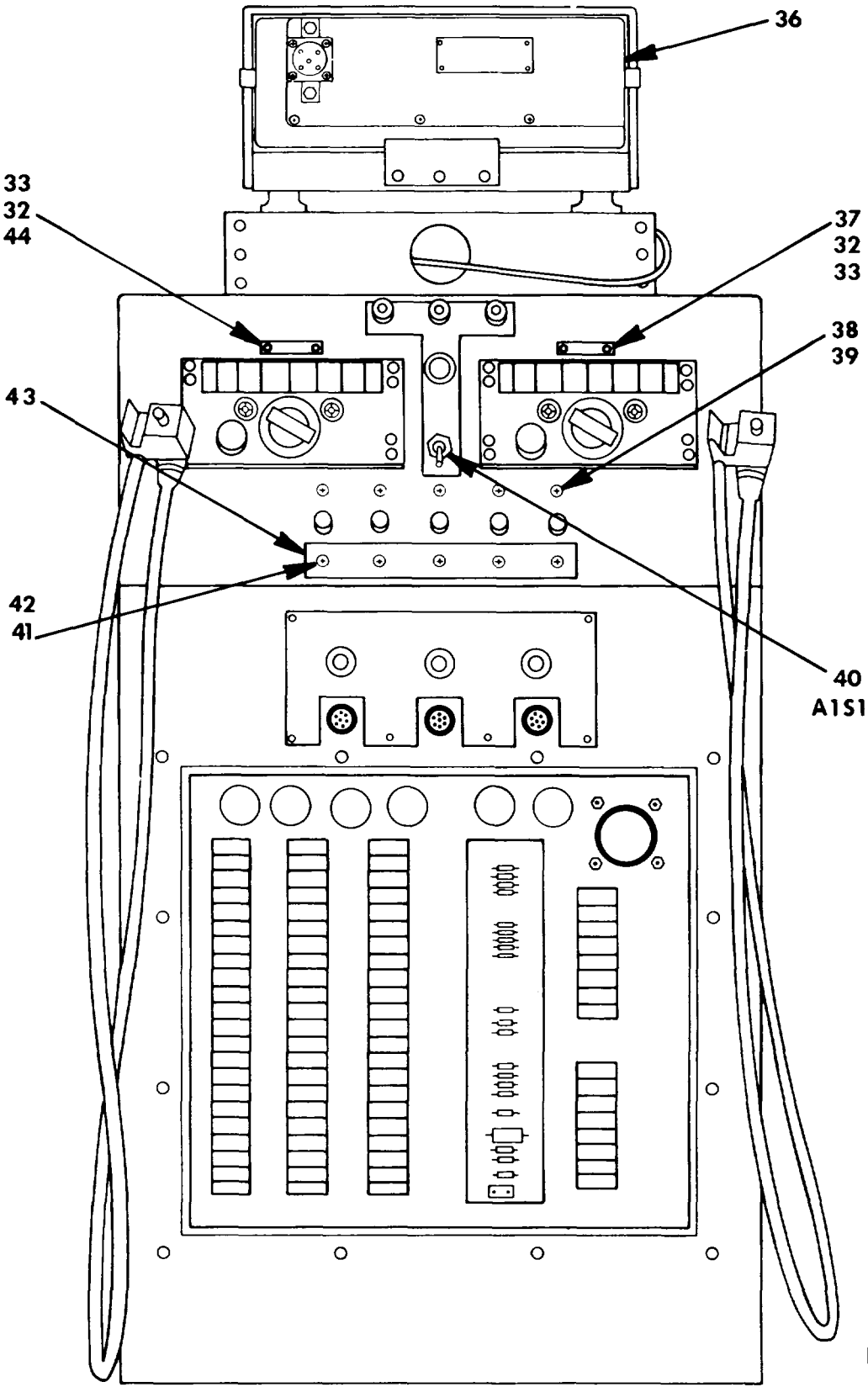
Figure 16. Frame Assembly (V)1 and 2 (Sheet 4 of 6).
